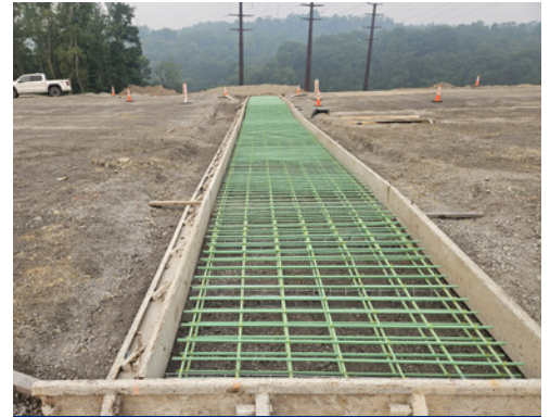
Approach sleeper slab construction - bridges over Camp Hollow Road.
