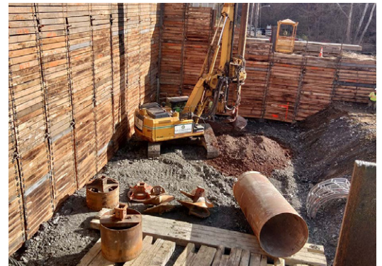
Pier foundation construction for the bridge over Camp Hollow Road.
