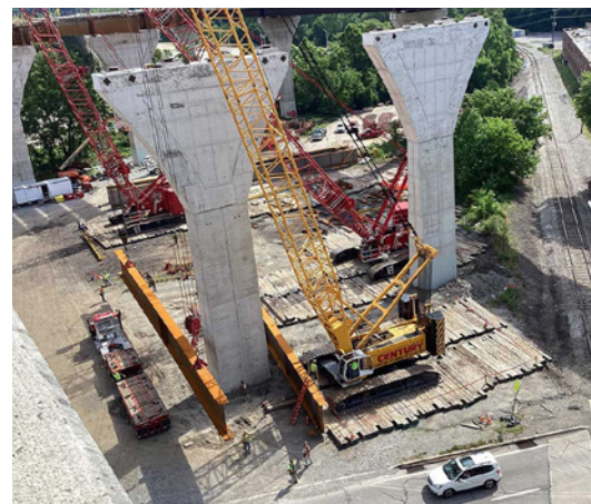
Steel girder placement for bridge spanning SR-51.
