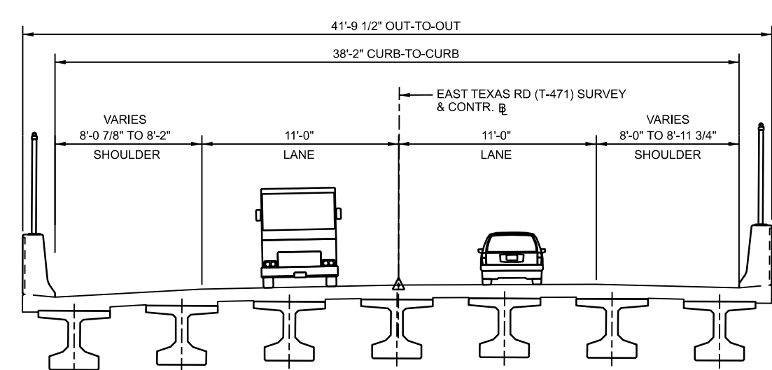
East Texas Road Proposed Bridge Typical Section
