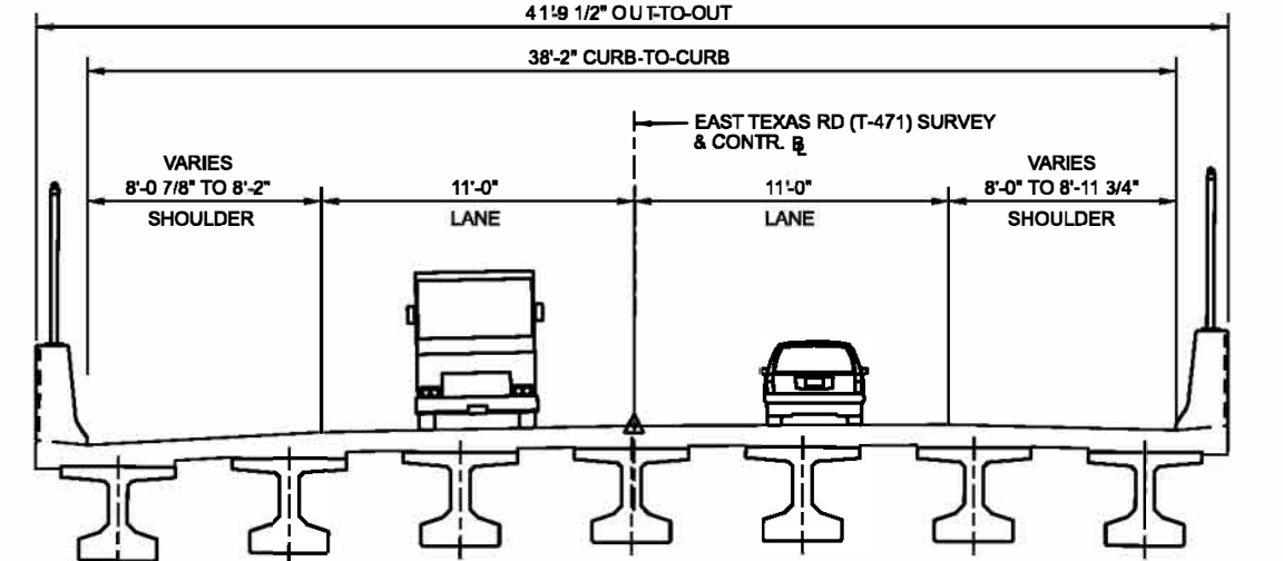
East Texas Road Proposed Bridge Typical Section
