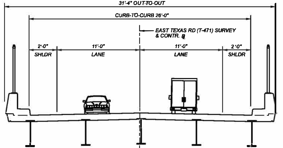
East Texas Road Existing Bridge Typical Section
