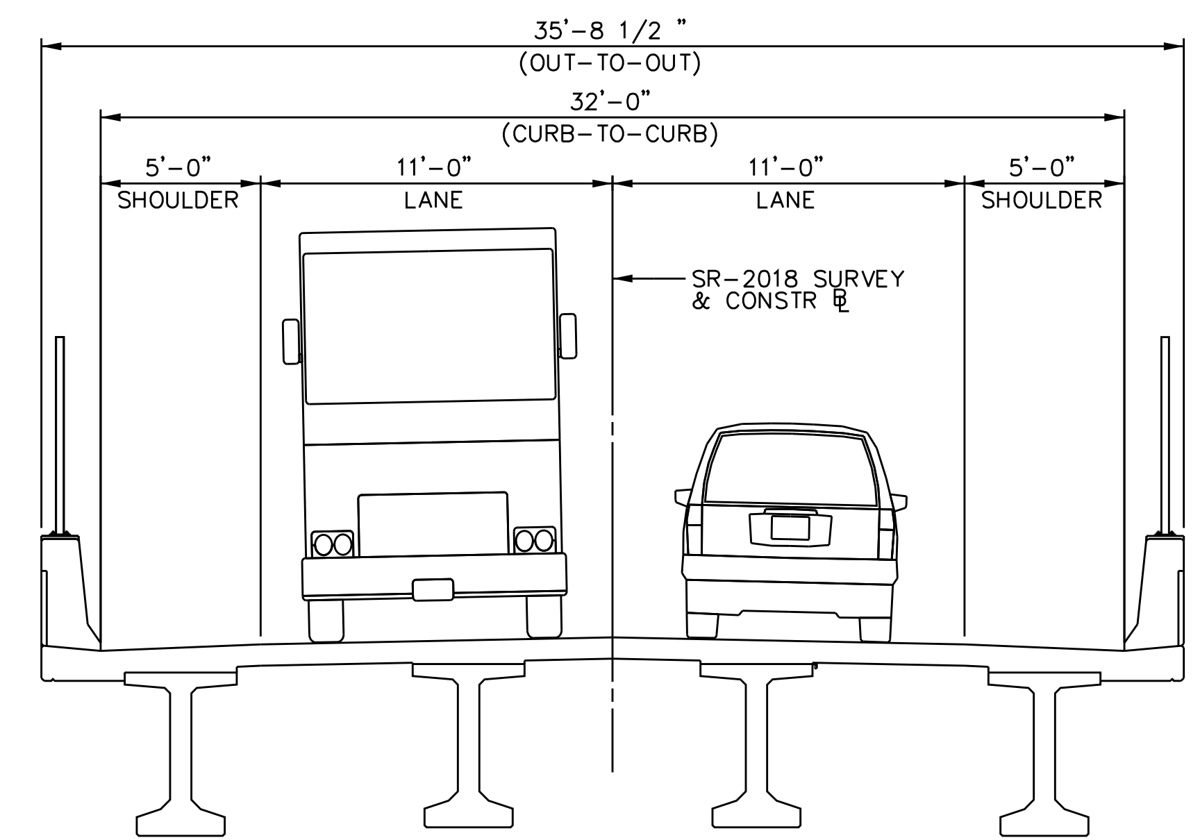
Vera Cruz Road Proposed Bridge Typical Section
