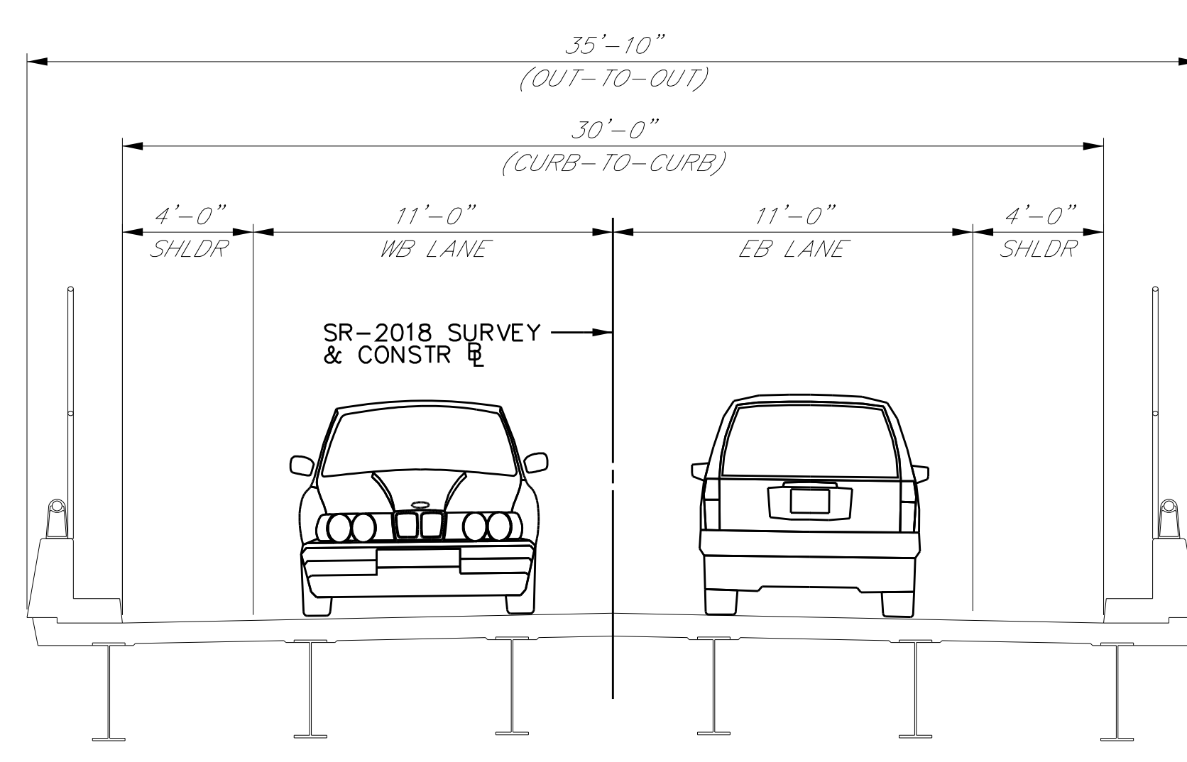
Vera Cruz Road Existing Bridge Typical Section
