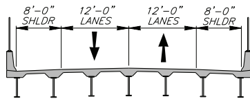
SR 380 EXISTING TYPICAL BRIDGE (LOOKING EASTBOUND)
