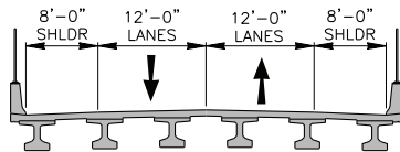
SR 380 PROPOSED TYPICAL BRIDGE (LOOKING EASTBOUND)
