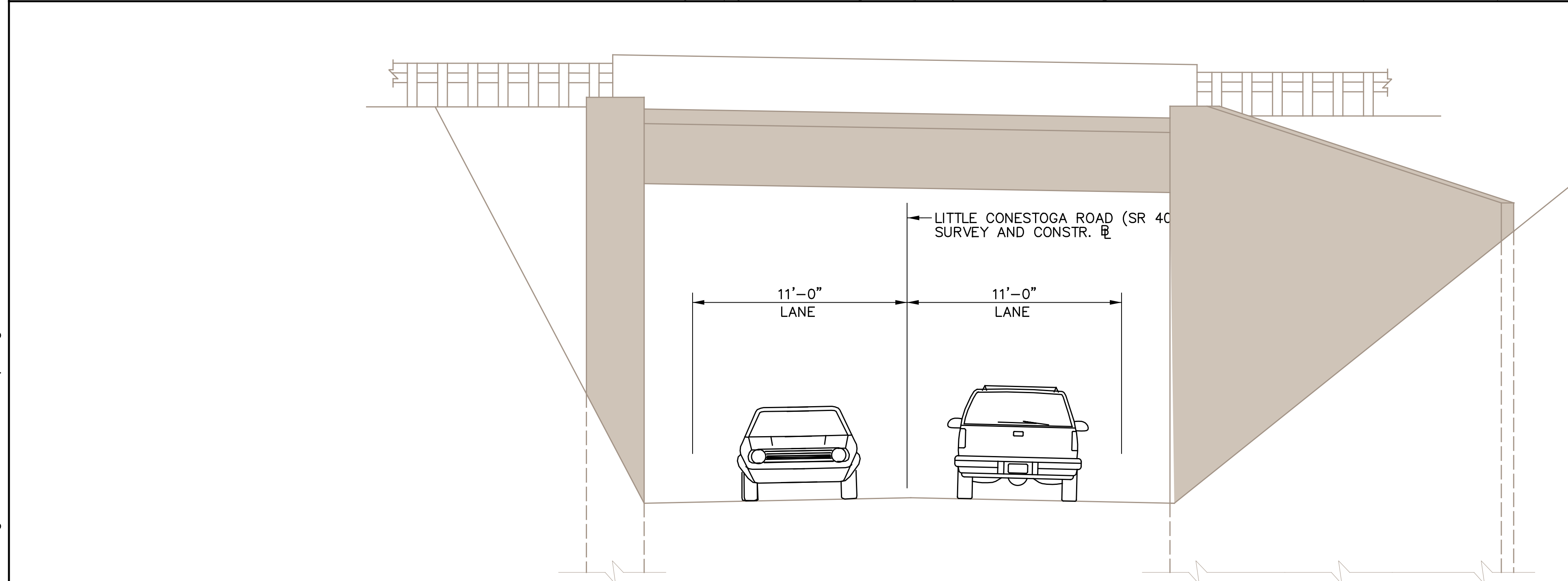
LITTLE CONESTOGA ROAD - EXISTING BRIDGE ELEVATION
