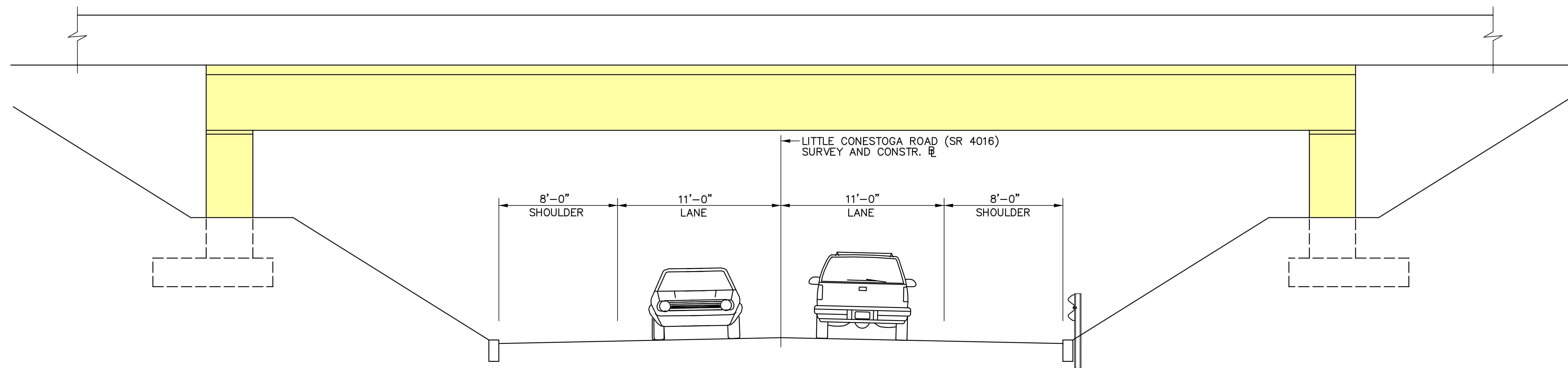
LITTLE CONESTOGA ROAD - PROPOSED BRIDGE ELEVATION
