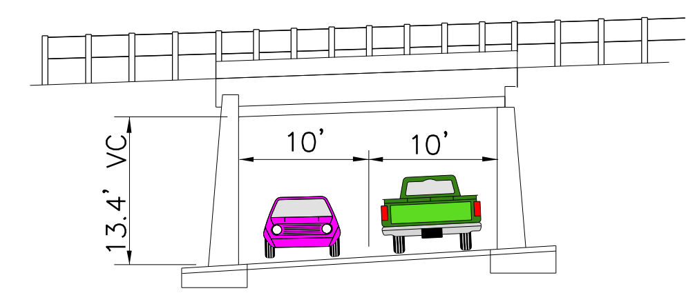
EXISTING SR 1004 TYPICAL SECTION
