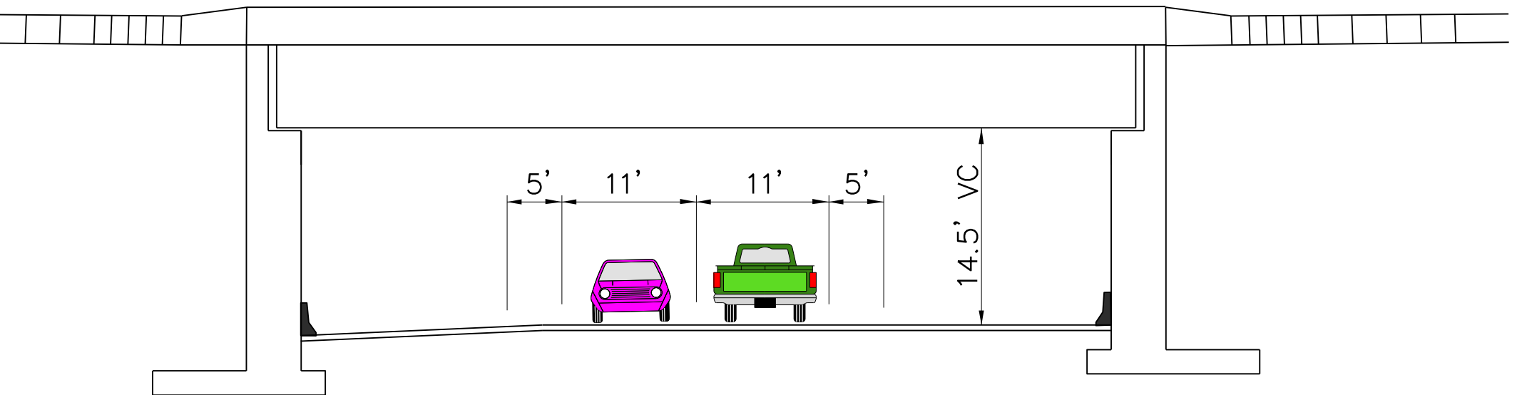
PROPOSED SR 1004 TYPICAL SECTION
