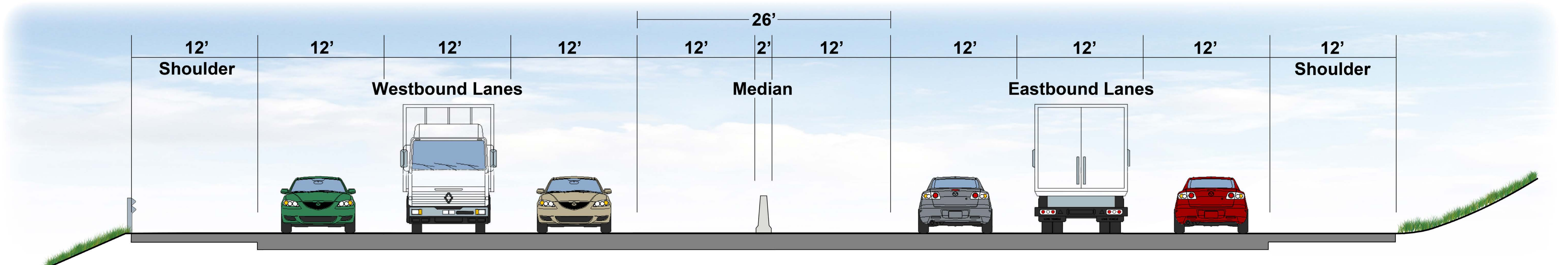
Proposed Typical Section Milepost 125.8 to Milepost 133.8
