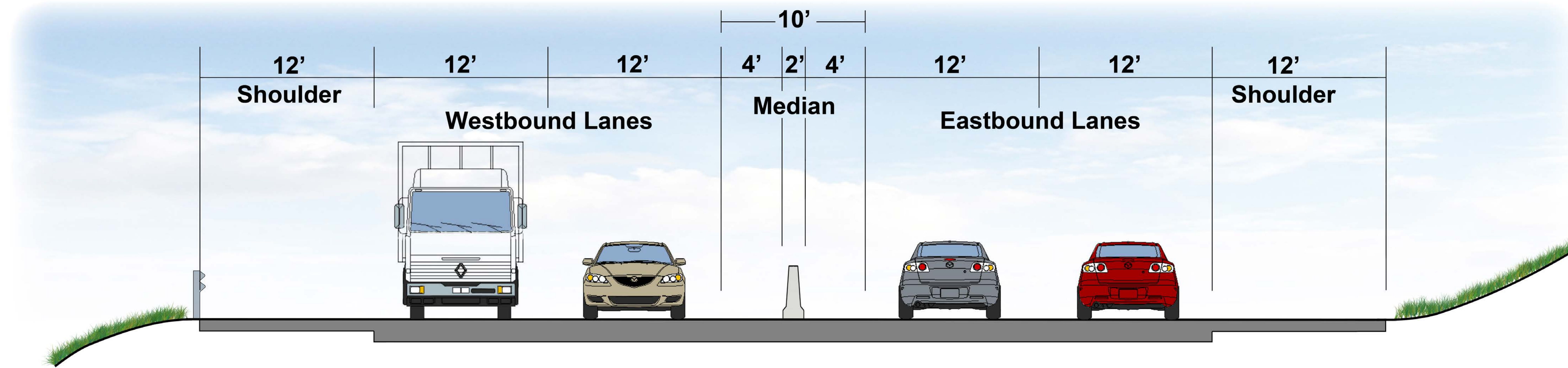
Existing Typical Section Milepost 129.0 to Milepost 133.8
