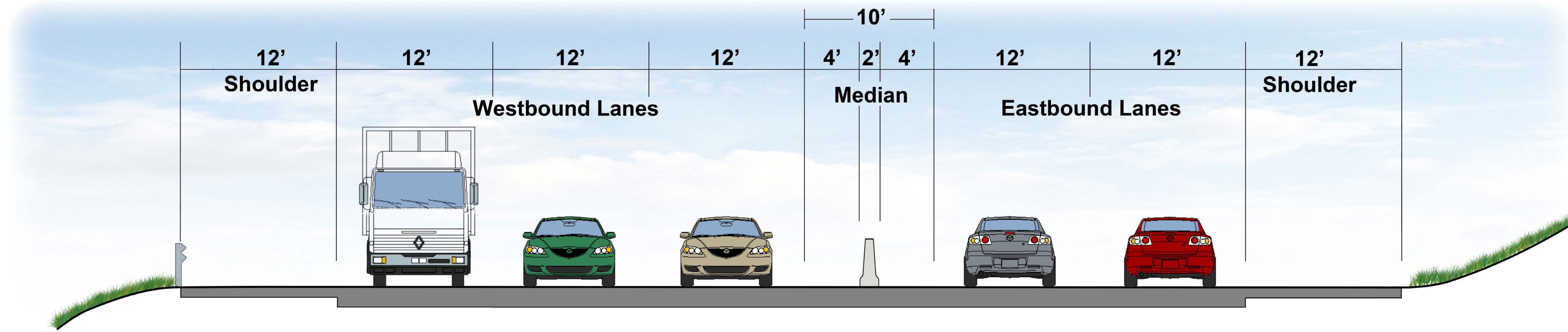
Existing Typical Section Milepost 125.8 to Milepost 129.0
