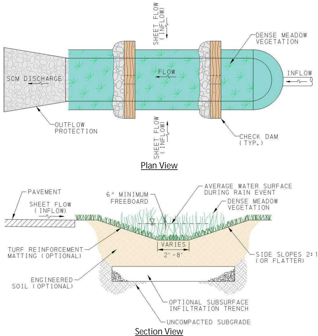
Figure 6.11.3: Vegetated Swale (VSW/VSC) - Common Elements
