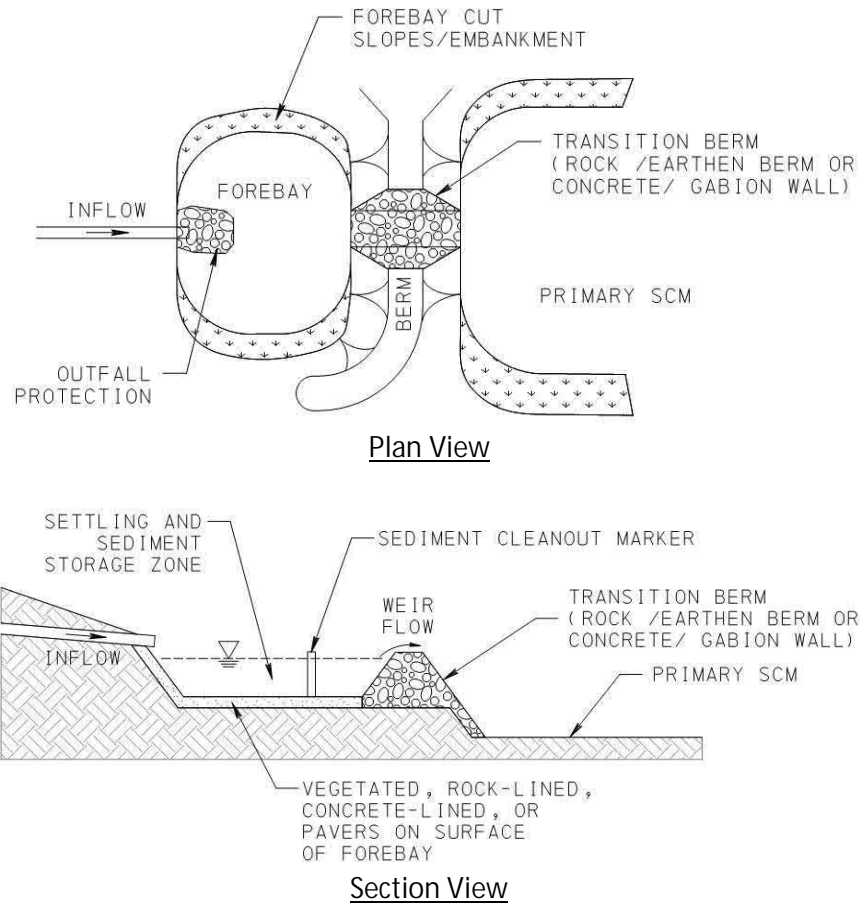
Figure 5.6.2: Forebay - Common Elements
