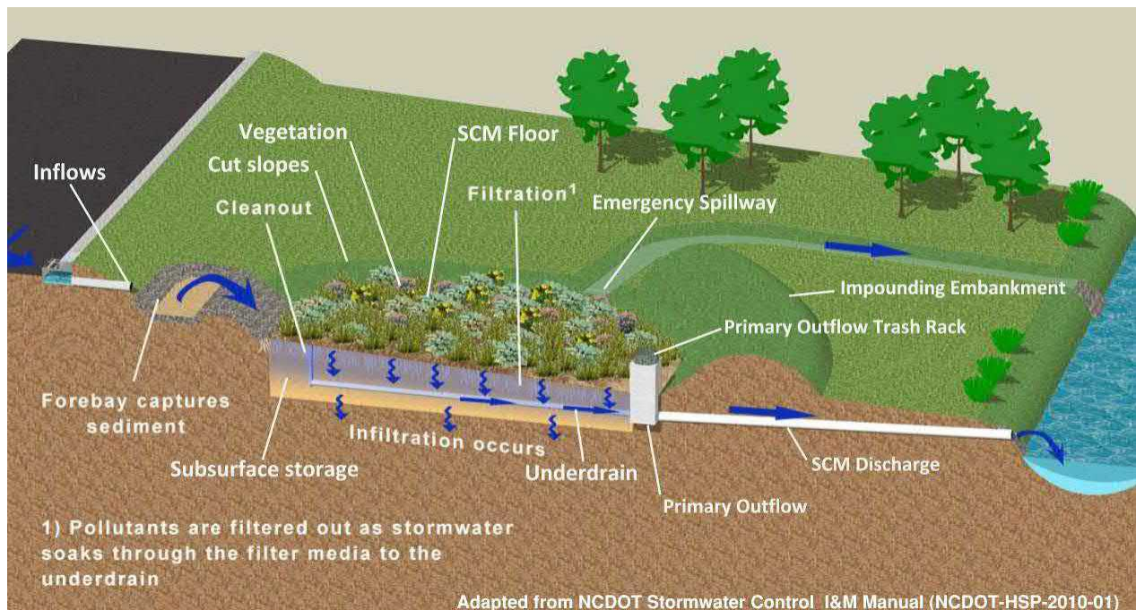
Figure 5.1.2: Anatomy of a Typical Surface SCM
