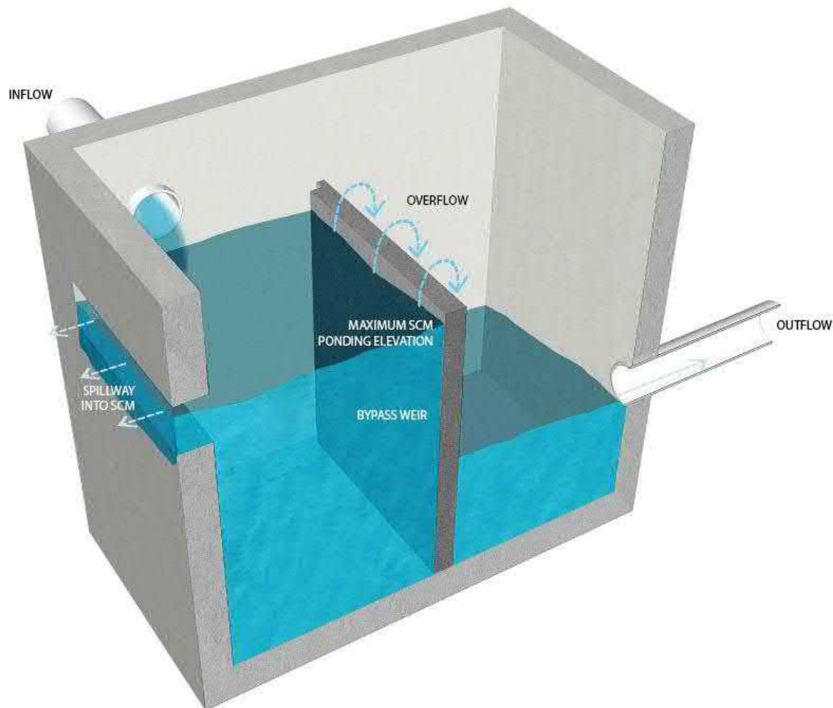
Figure 5.5.1: Flow Splitter
