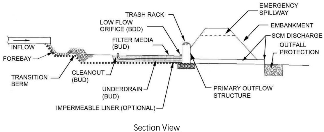
Figure 6.1.2: Dry Basins - Common Elements (Adapted from NCDOT-HSP-2010-01)
