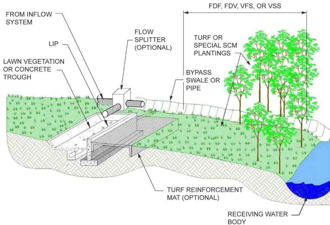
Figure 6.14.2: Surface LSO - Common Elements (Adapted from NCDOT-HSP-2010-01)
