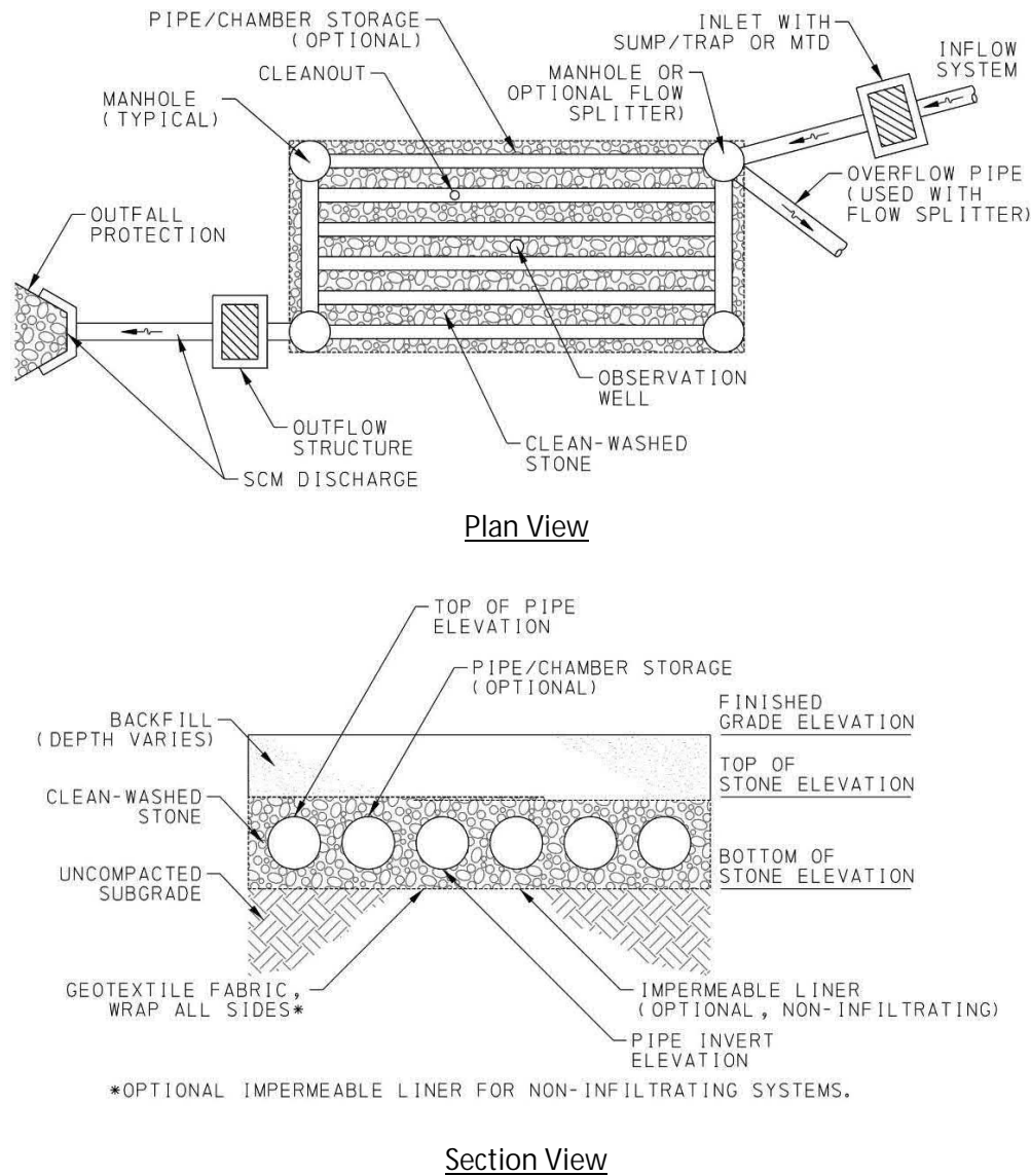
Figure 6.6.2: Subsurface Detention Storage - Common Elements
