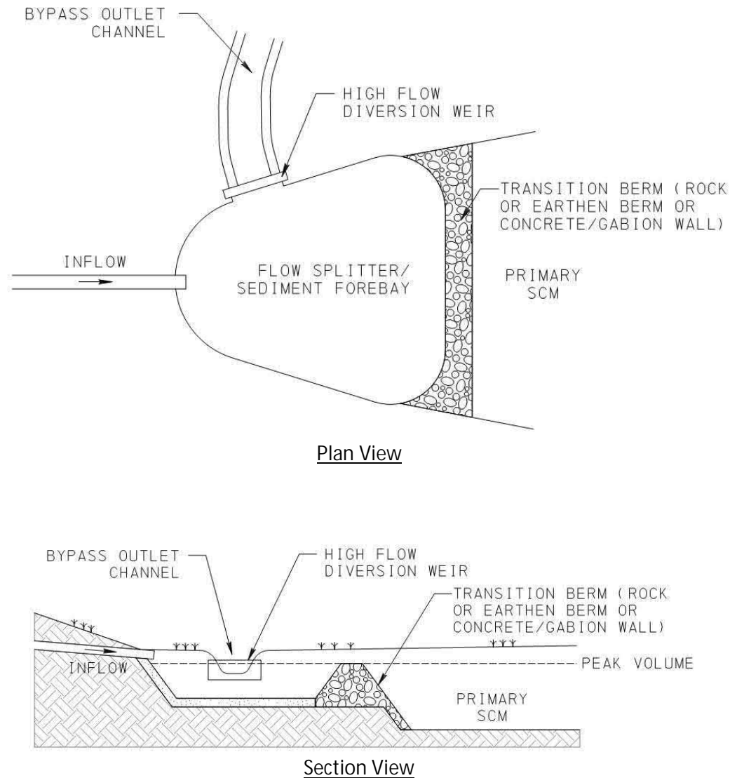
Figure 5.5.3: Surface Flow Splitter – Common Elements
