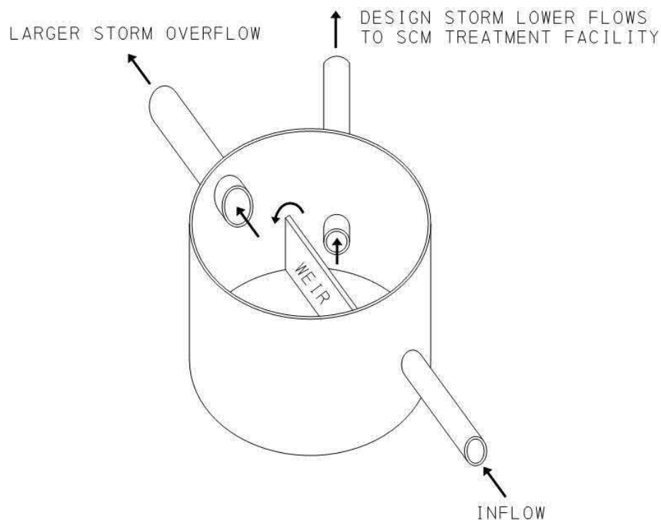
Figure 5.5.2: Subsurface Flow Splitter – Common Elements
